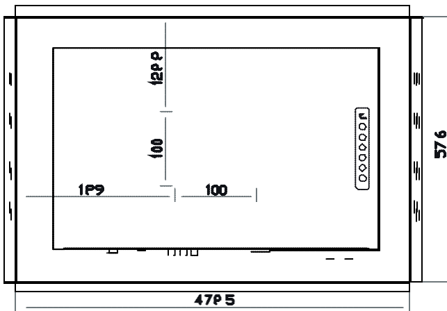
Rear View
