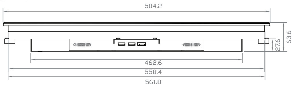
Bottom View
