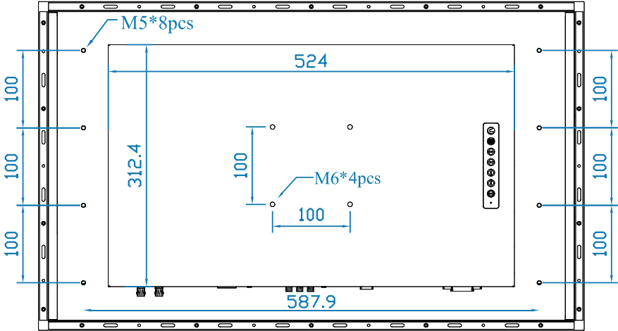
Rear View
