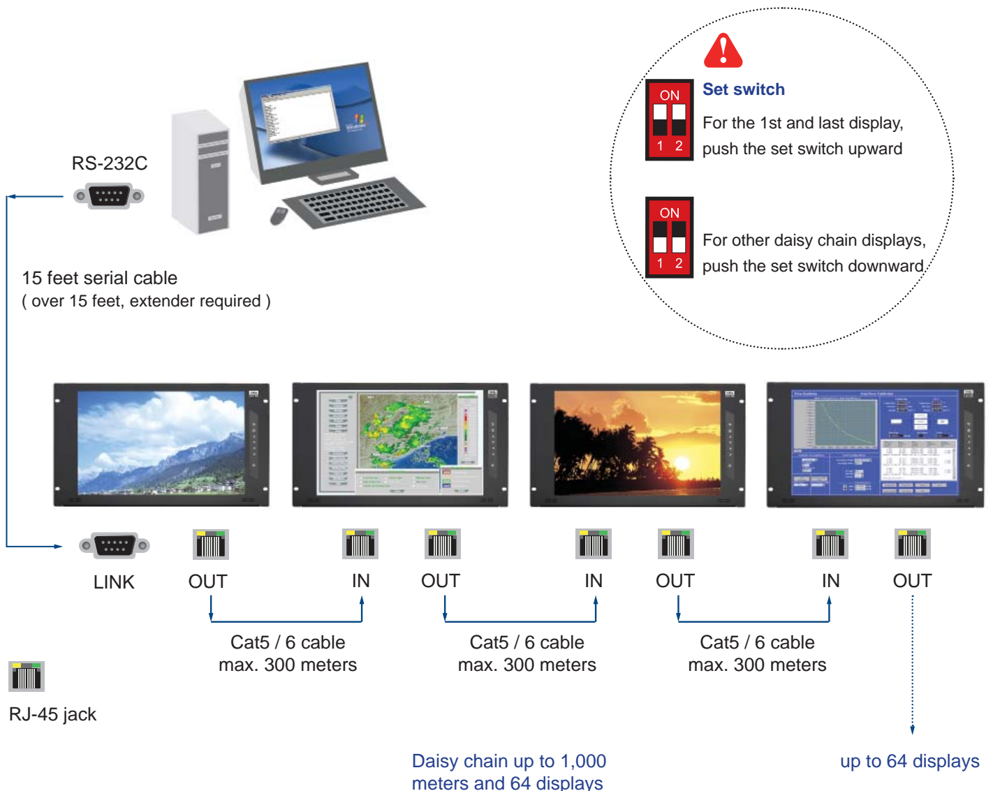
Fig. 1-1 Connecting the PC & LCD Displays
